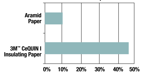
Moisture Absorption
