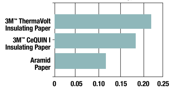
Varnish Absorption
